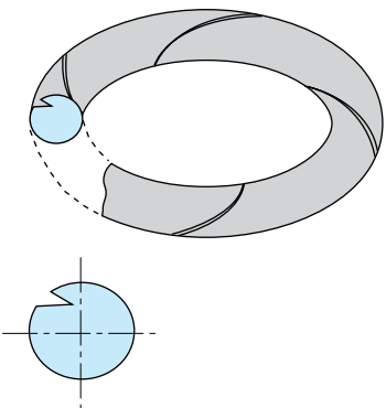
Picture of a spiral failure O-ring
